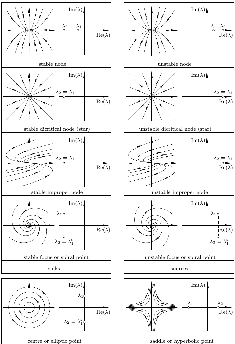
Fig. 3.1.8: Survey of the singularities in a two-dimensional phase space, phase portraits and eigenvalues for n=2
