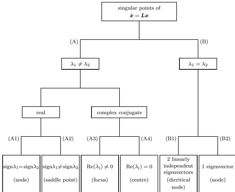
Fig. 3.1.1: Survey of the eigenvalues of singular points for n=2
